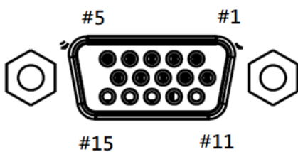
15 Pin D-sub Connector
