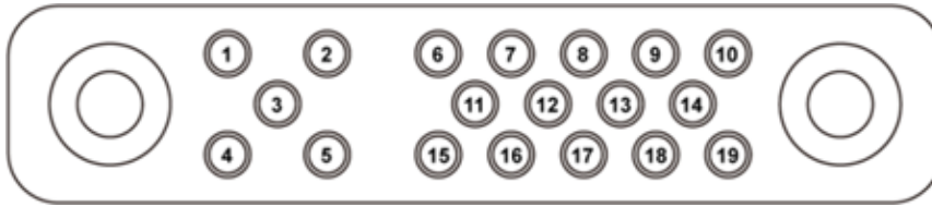
19 Pin Docking Connector
